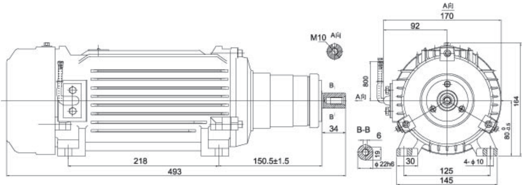
安装及外形尺寸 Overall Dimensions
